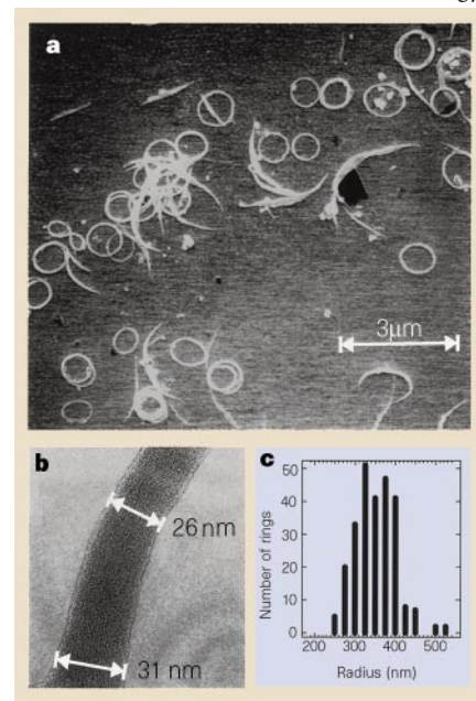
Figure 1 Ring formation in single-walled carbon nanotubes. a , Scanning electron micrograph of a SWNT sample dispersed on a hydrogen-passivated silicon substrate, with rings clearly visible. Rings are produced by mixing long SWNTs with a solution of concentrated sulphuric acid and hydrogen peroxide and irradiating them with ultrasound for 1–3 h (40 kHz, 190 W) at 40–50° C, which disperses them and shortens the nanotube ropes 5 . After sonication, the solution is filtered through a 0.2- \mu\text{m} membrane filter, and the residue dried and suspended in 1,2-dichloroethane with a brief period of sonication. A high yield requires shortening the raw nanotubes to a length of 2–4 \mu\text{m} . Yield varies with time of exposure to ultrasound and concentration of peroxide solution. b , TEM image of a section of a ring wall (courtesy of L. Gignac). c , Histogram showing the distribution of ring radii.
