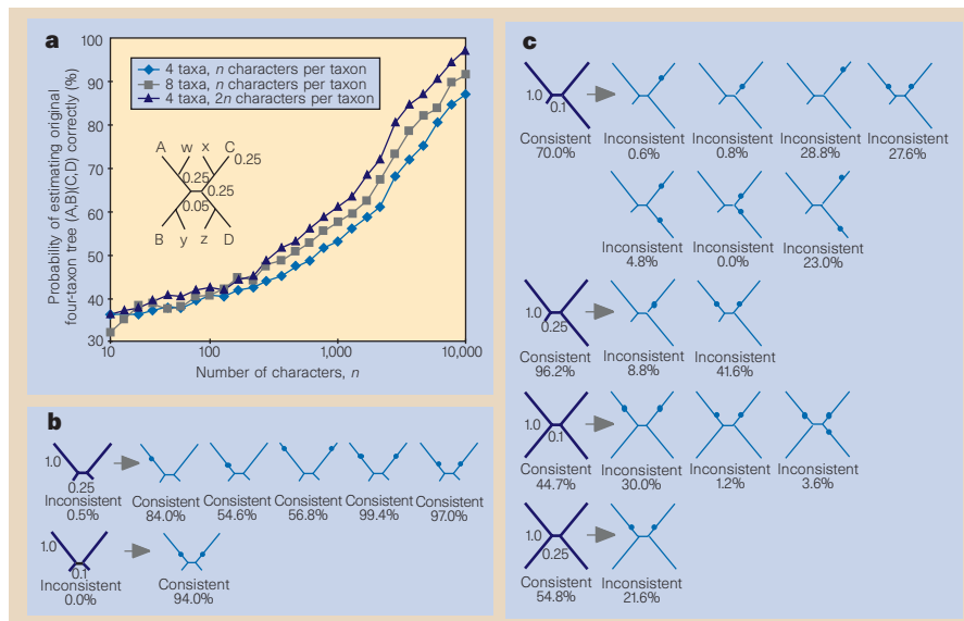
Figure 1 Modelling of phylogenetic strategies. Character data were generated on trees according to a two-state homogeneous, reversible Markov model 9 . Branch lengths are the expected number of changes per character. Trees are unrooted because determining the location of the root requires extrinsic information. PAUP version 4.0 was used for all analyses 10 . a , For some phylogenies that are difficult to estimate, adding characters is better for accuracy than adding taxa. Parsimony was used to estimate the relationships of A, B, C and D alone or including taxa w, x, y and z. All points are means for 1,000 simulations. b , c , Effect of long-branch subdivision on the accuracy of phylogeny reconstruction using parsimony, according to consistency and finite data simulation analyses. Bold indicates four-taxon trees for which adding taxa to long branches changed the estimation of relationship of those four taxa from inconsistent to consistent or vice versa. Trees on the right show the 19 (out of 288) cases where adding taxa affected the consistency of the estimation of relationships for the original four-taxon tree. The expected length of each tree is determined from the pattern frequencies predicted under the model and branch lengths. A consistent estimate is achieved if the expected length of the true tree is shorter than that of all others. Percentages refer to the number of times the correct relationships of the original four taxa were recovered in 500 replicate simulations of 5,000 characters. For trees with more than four taxa (all trees where taxa were added), characters were evolved and phylogenetic analyses were run using all taxa, after which 'added' taxa were pruned and resulting four-taxon trees were compared to the true tree. Trees shown are true (not estimated) trees. Dots show where taxa were added. b , Cases where long-branch subdivision caused a change from inconsistent estimation to consistency. c , Cases where long-branch subdivision caused a change from consistent estimation to inconsistency.
